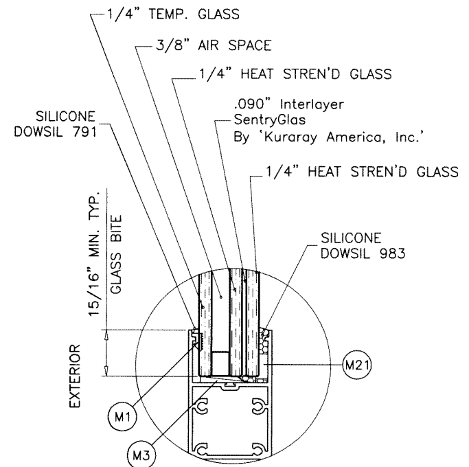
GLASS TYPE 'B' 1-1/4" OVERALL INSUL. LAM. GLASS
